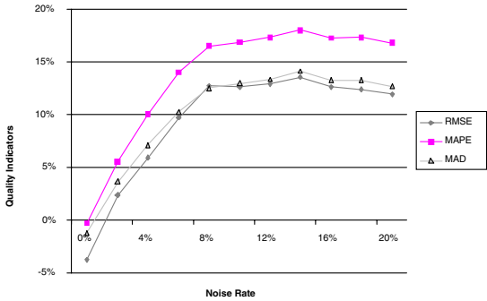
Fig. 2. Relative quality gain with autos when there is from 0 to 20% of noise.
