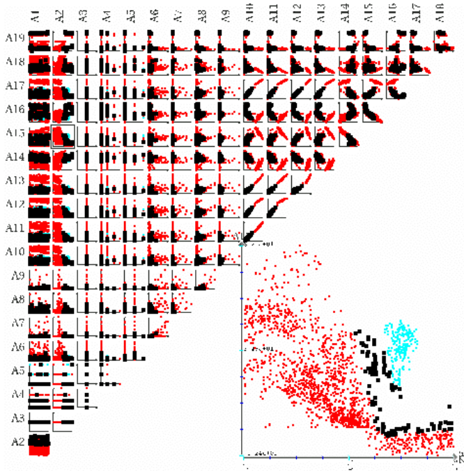
Fig. 4. Interactive selection of support vectors (in black).
