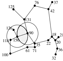
Fig. 1. RNG built with two numerical predictive attributes. Examples with the values 90 and 150 are connected because the lune (in gray) between these examples is empty.
