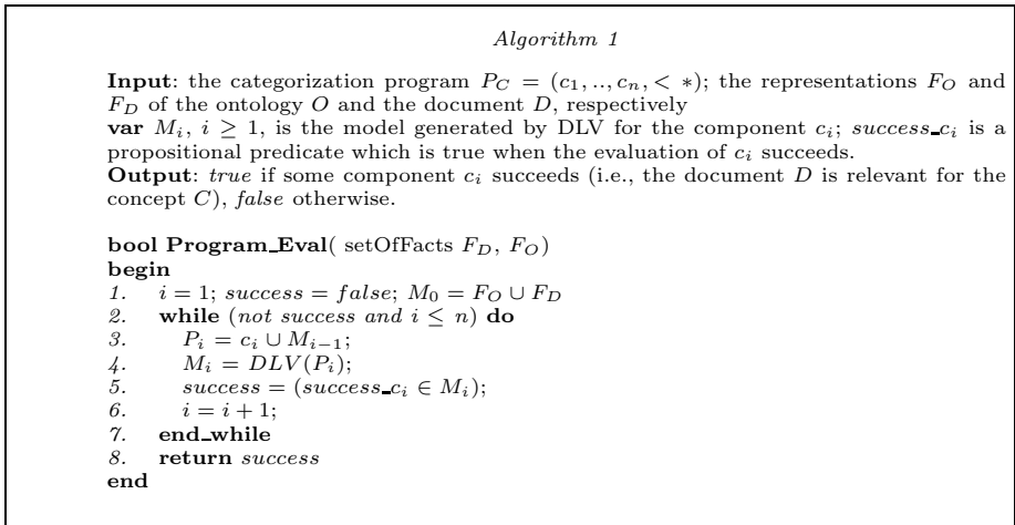
Fig. 2. The Categorization Program Evaluation Algorithm.
