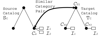
Fig. 1. An example of a learned rule.
