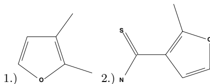
Fig. 6. A 2D graphical representation of an example rules found by SMIREP. Pattern 1 was found in the AM experiment. The rule contained only one single pattern (‘Cc1ccoc1C’). Pattern 2 was found in AI experiment. The rule contained only one single pattern (‘NC(=S)c1ccoc1C’).
