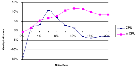
Fig. 3. Relative RMSE reduction for the CPU database as a function of the noise rate with a logarithmic transformation ( ln CPU ) – or not ( CPU ) – of the class attribute Y .
