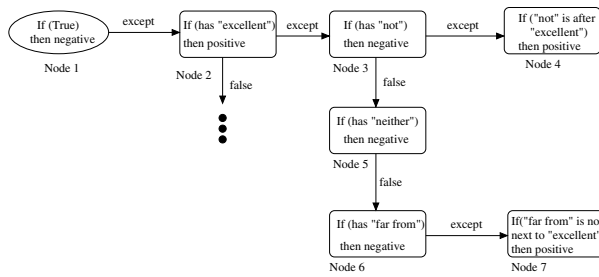
Fig. 1. An example SCRDR tree with simple rule language to classify a text into positive or negative class. Node 1 is the default node. A text that contains excellent is classified as positive by Node 2 as long as none of its exception rules fires, i.e., the text does neither contain not , neither nor far from so Node 3,5,6 would not fire. A text that has not excellent is classified as negative by Node 3 while it is classified as positive by Node 4, if it contains excellent but not . If it contains far from excellent then it is classified as negative by Node 6.
