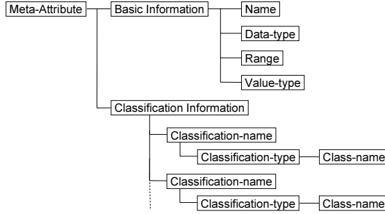
Fig. 1. Definition of the meta-attribute.
