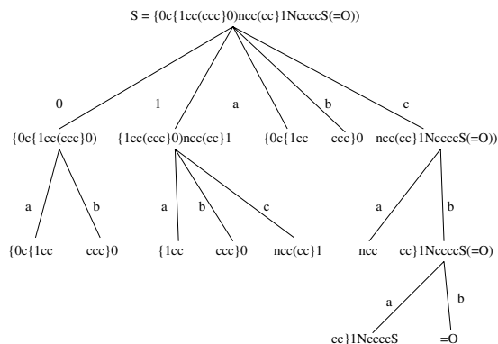
Fig. 4. The resulting fragment tree given the SMILES string S = 'c1c2c(ccc1)ncc(cc2NccccS(=O))' .
