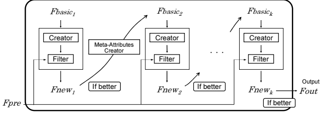
Fig. 6. Outline of Phase.
