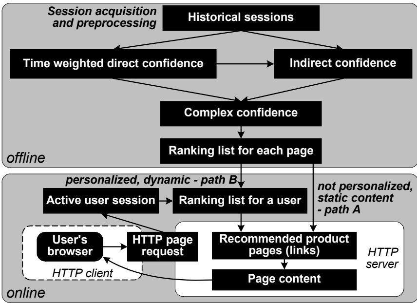
Fig. 4. Method overview.
