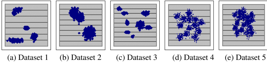
Fig. 2. Synthetic datasets.
