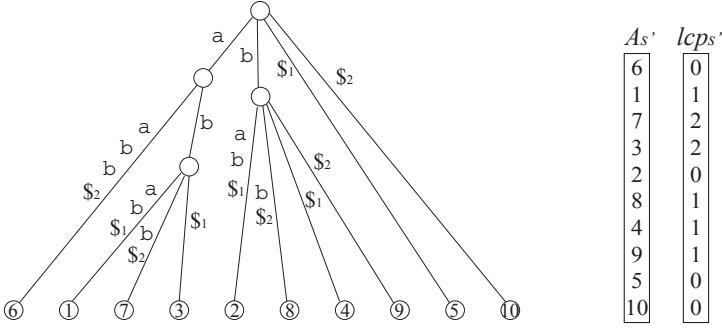
Fig. 2. The tree is the GST for set \{\mathbf{abab}, \mathbf{aabb}\} . Each leaf y is labeled by \text{pos}(y) with respect to the concatenated string s' = \mathbf{abab}\$1\mathbf{aabb}\$2 . The left and right arrays are the suffix and lcp arrays of string s' , respectively.
